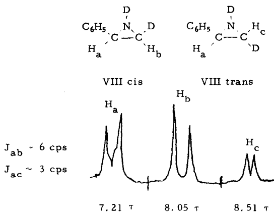
Fig. 1. NMR Spectrum of a Mixture of VIII cis and VIII trans
